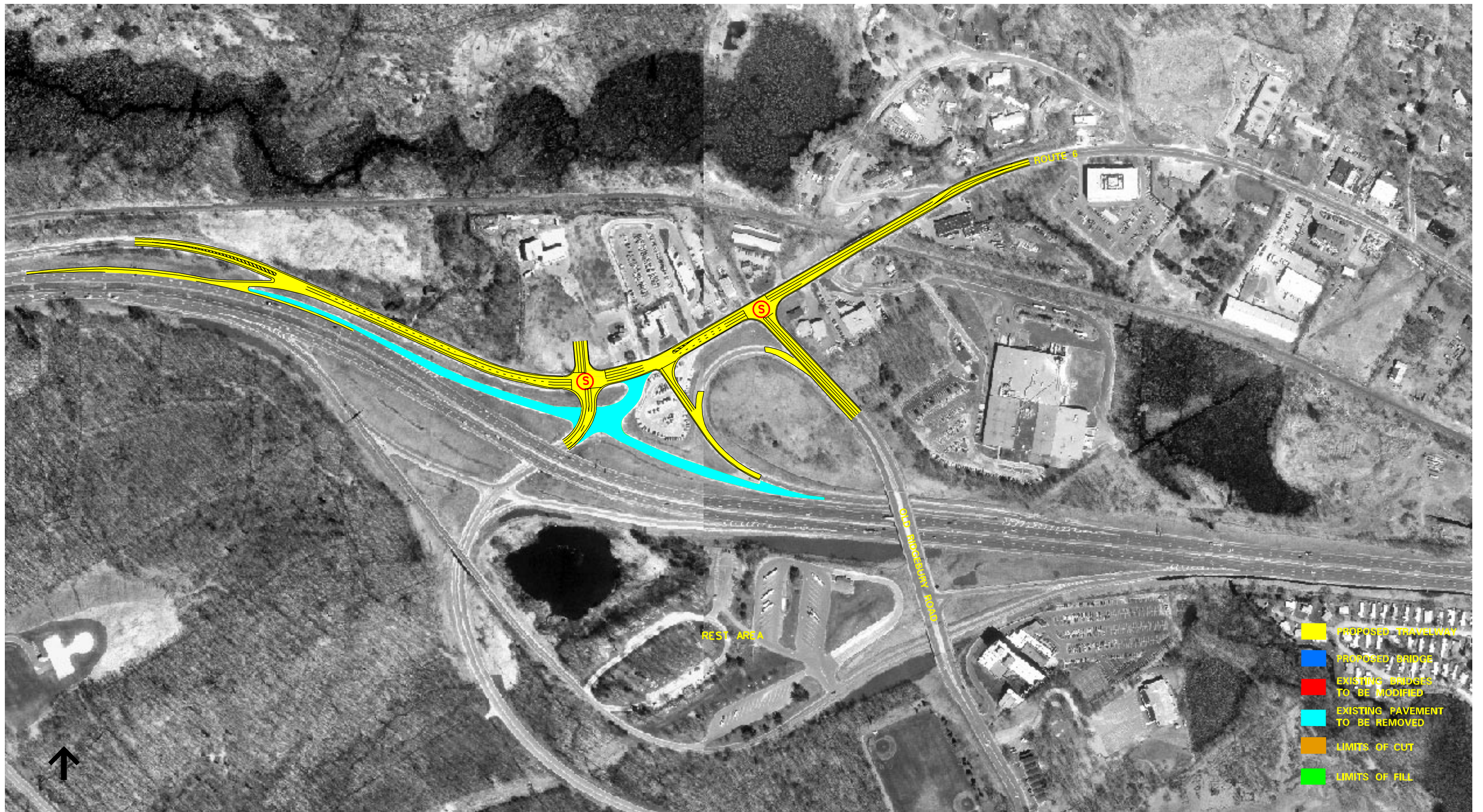
Figure 6-3 Exit 2 Long-Term Improvements
