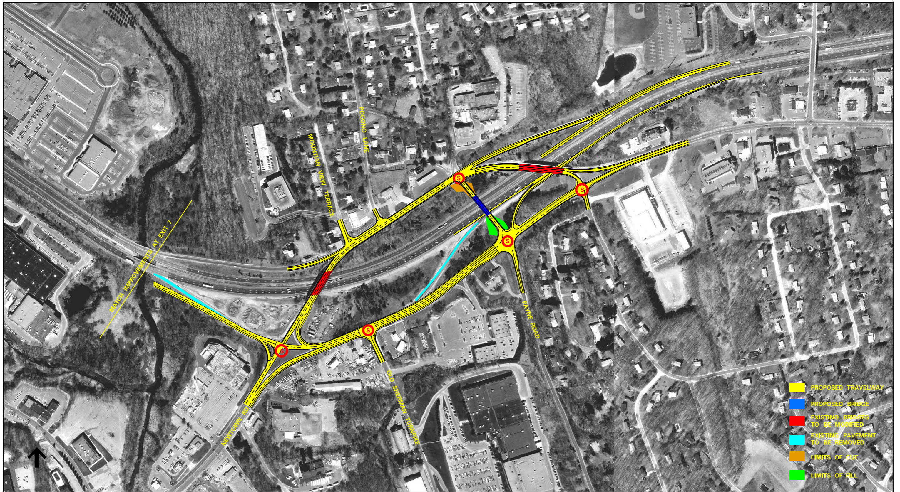
Figure 6-14 Exit 8 Long-Term Improvements
