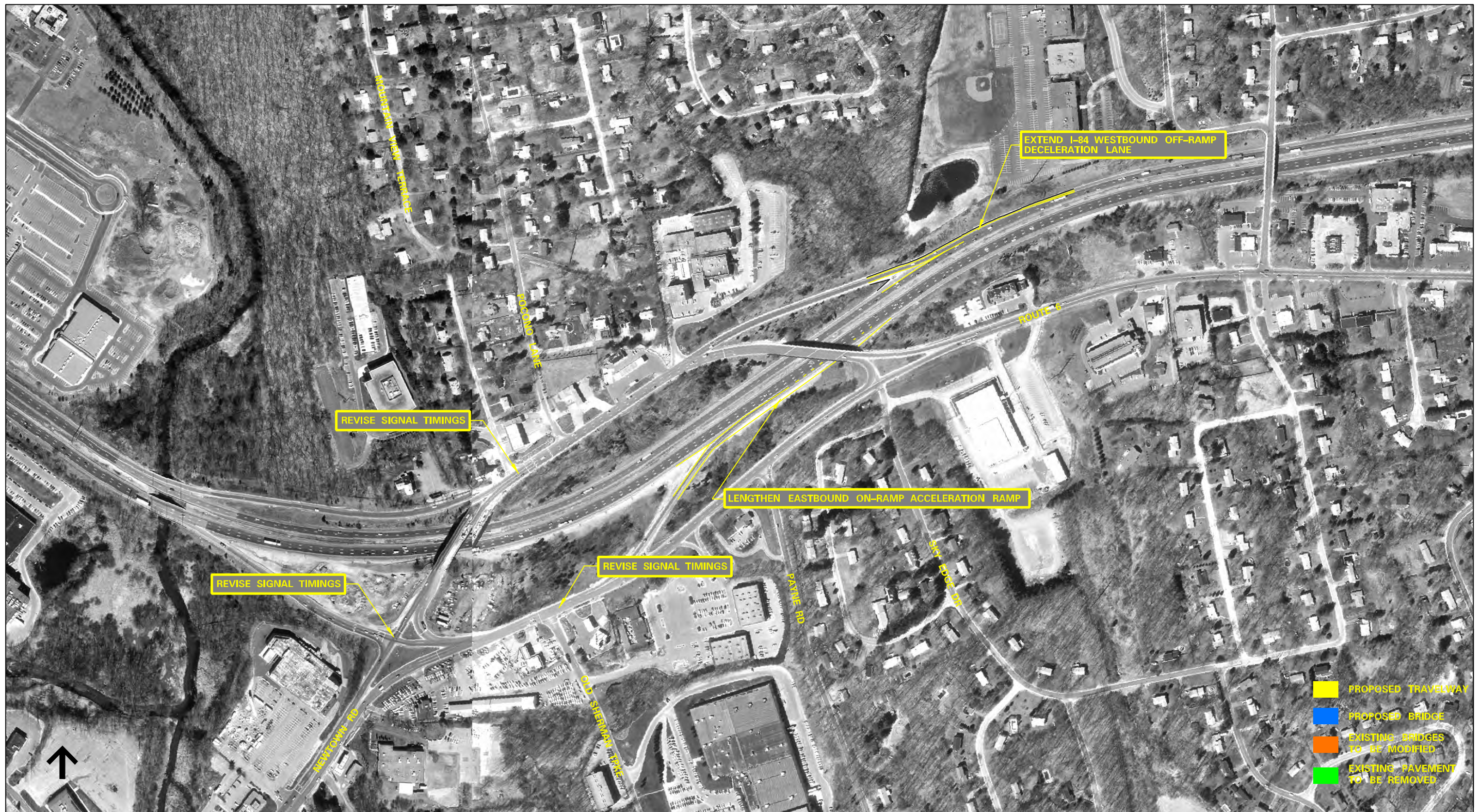
Figure 6-11 Exit 8 Short-Term Improvements
